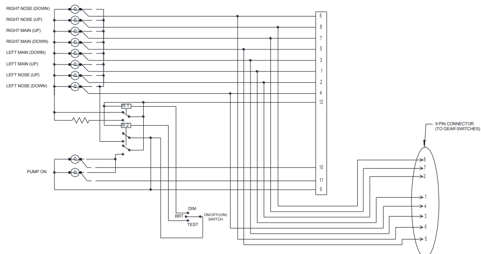
ELECTRICAL SCHEMATIC
