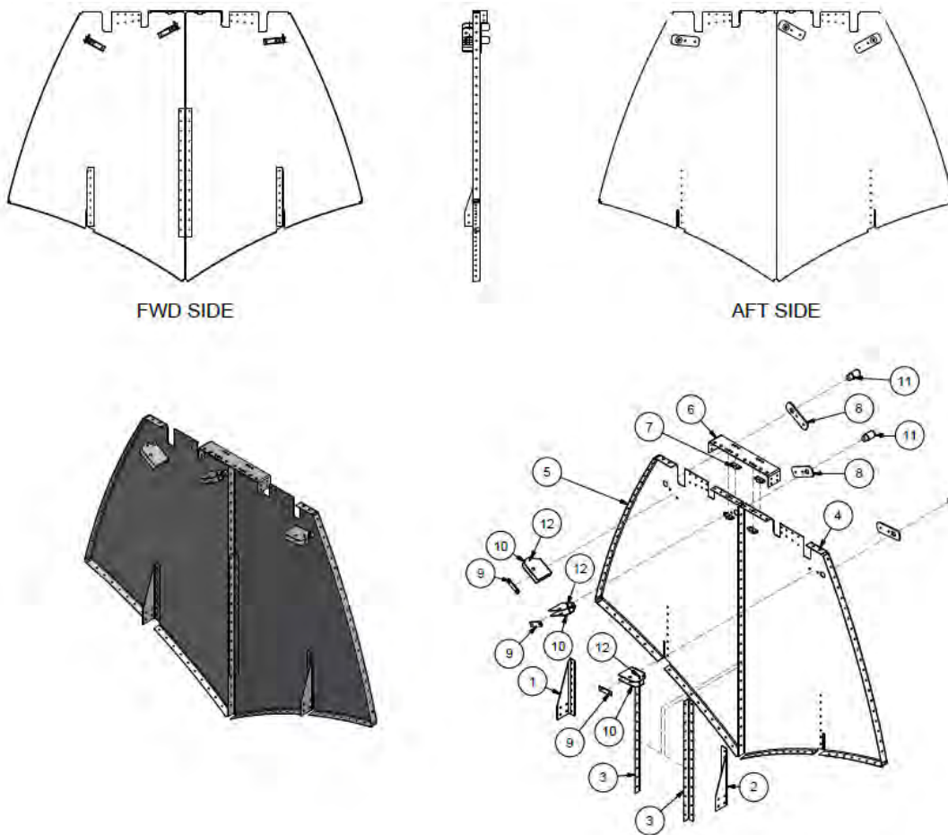
PARTS LIST ASS'Y., BULKHEAD 12, LEFT FLOAT
