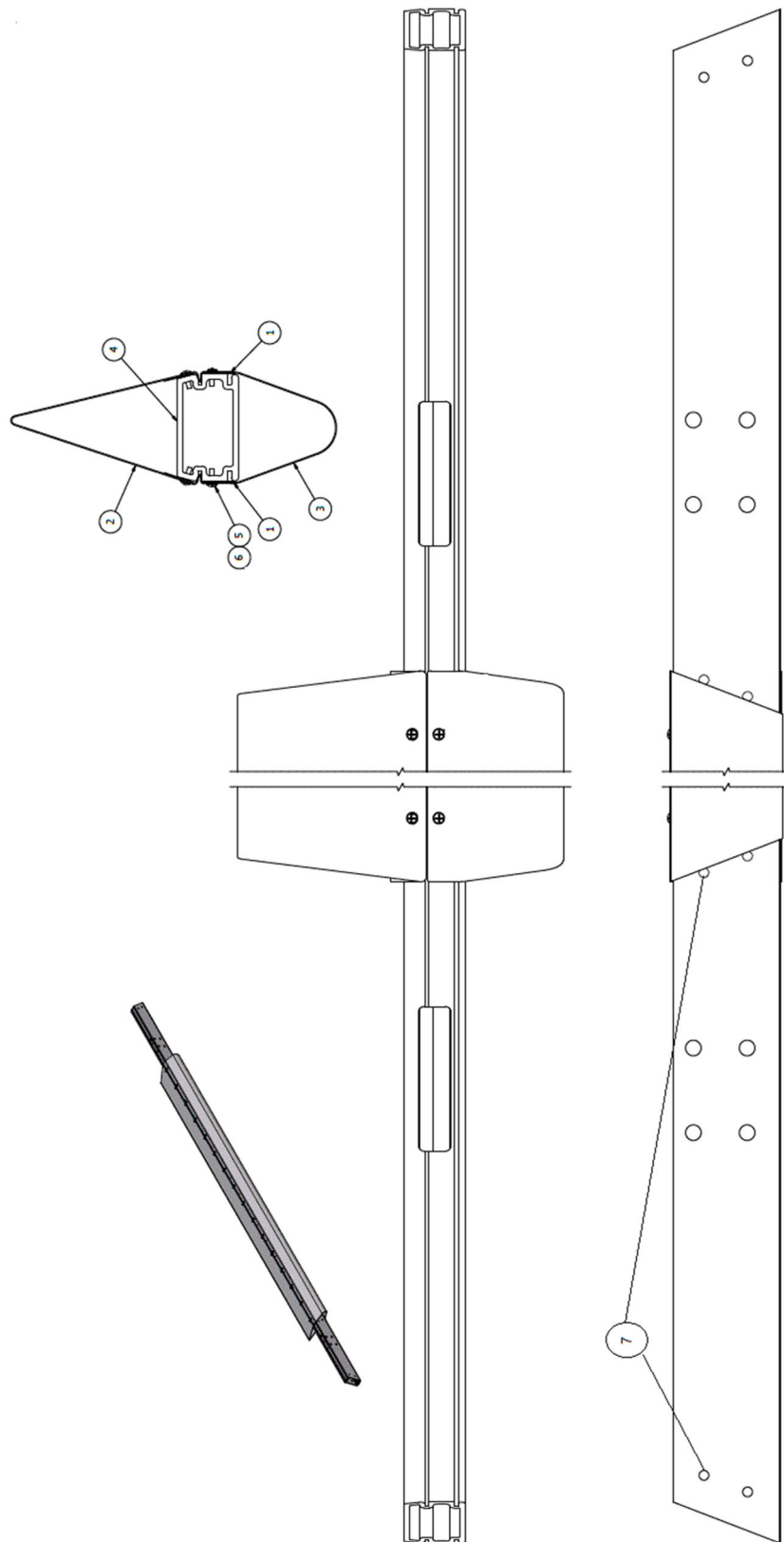
INSTALLATION AND ASSEMBLY - SPREADER BAR, AFT FIGURE 15
