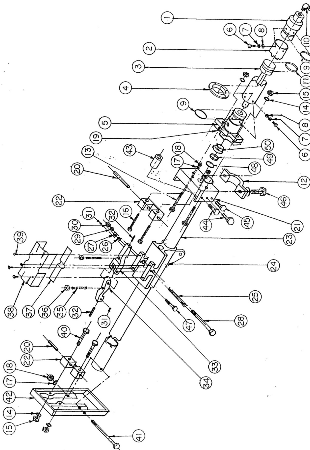
MAIN GEAR SLIDE TUBE ASS'Y (O-RINGS INSTALLED)
