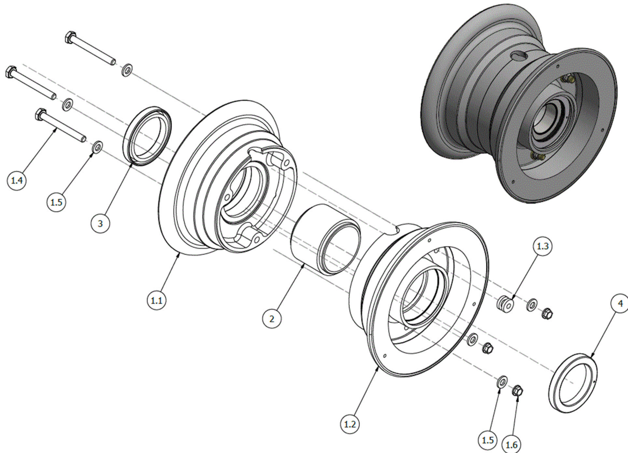
ASS'Y, NOSE WHEEL WITHOUT TIRE
