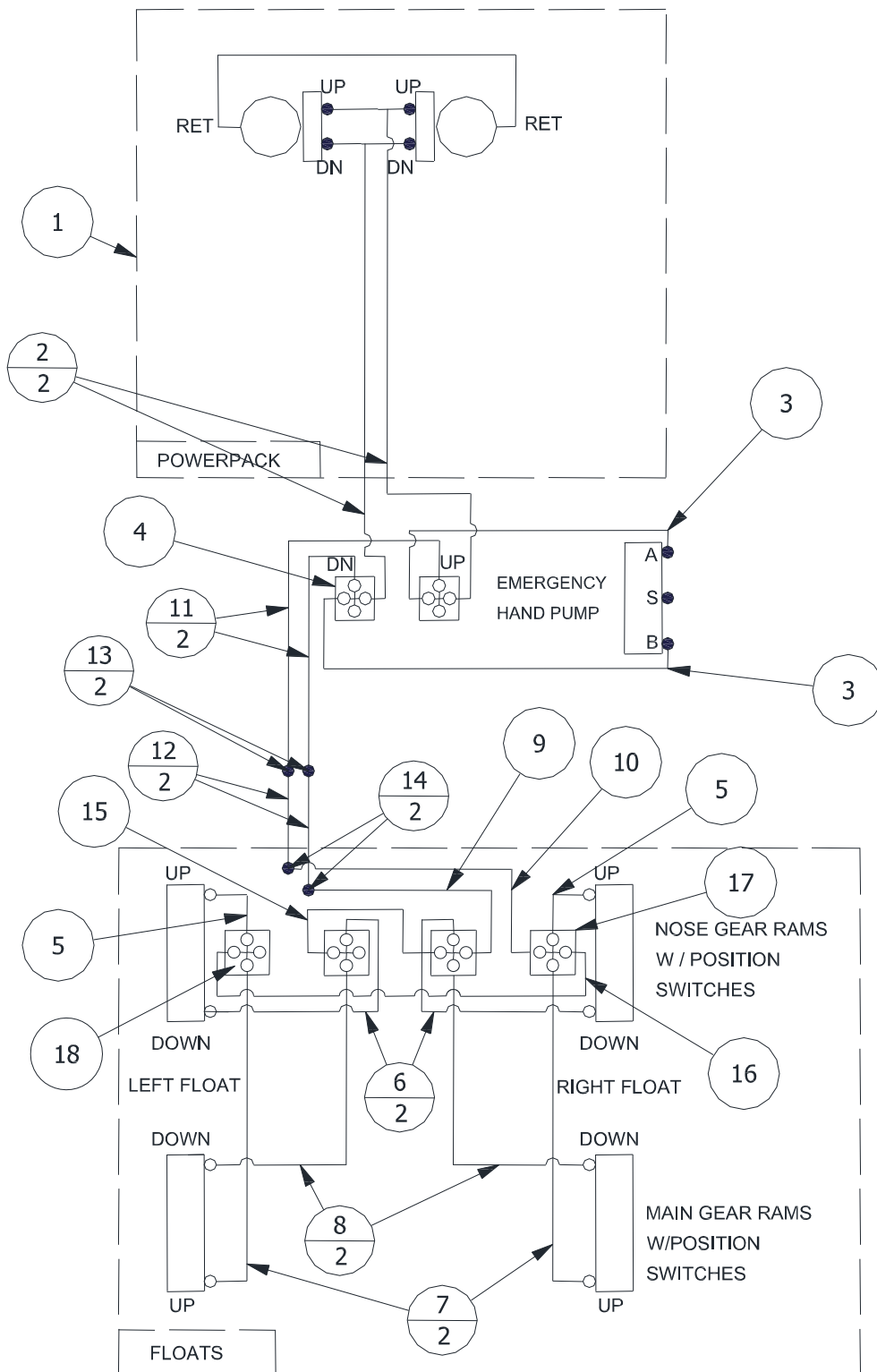
HYD. SYSTEM SCHEMATIC – AMPHIBIAN
