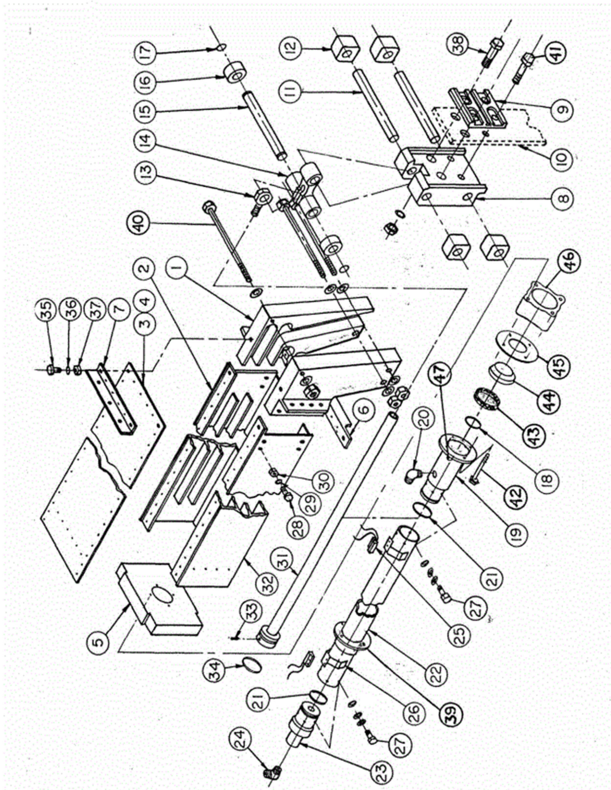
NOSE GEAR RETRACTION ASS'Y., UPR. END (O-RINGS INSTALLED)
