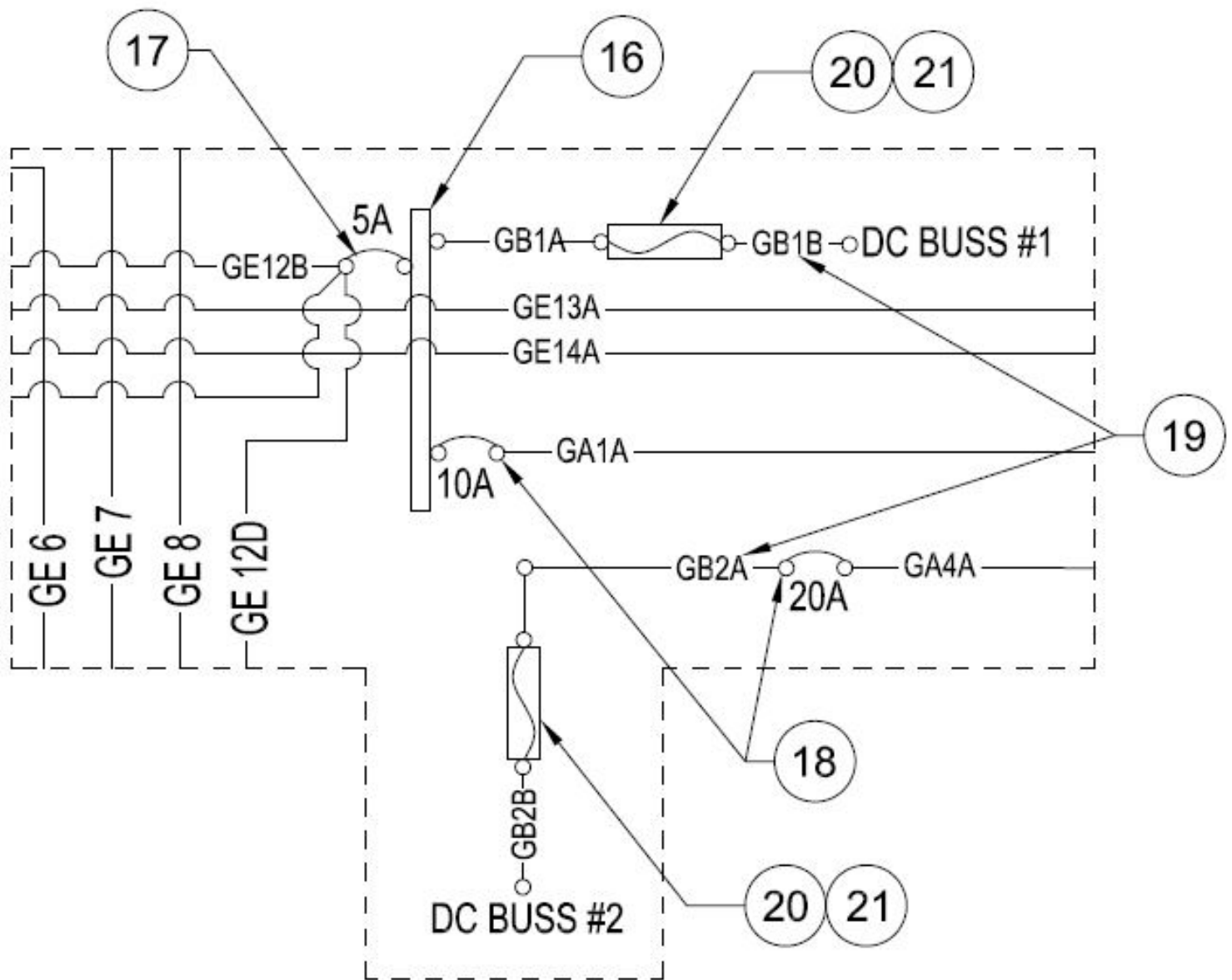
CIRCUIT BREAKER CONFIGURATION "B"
