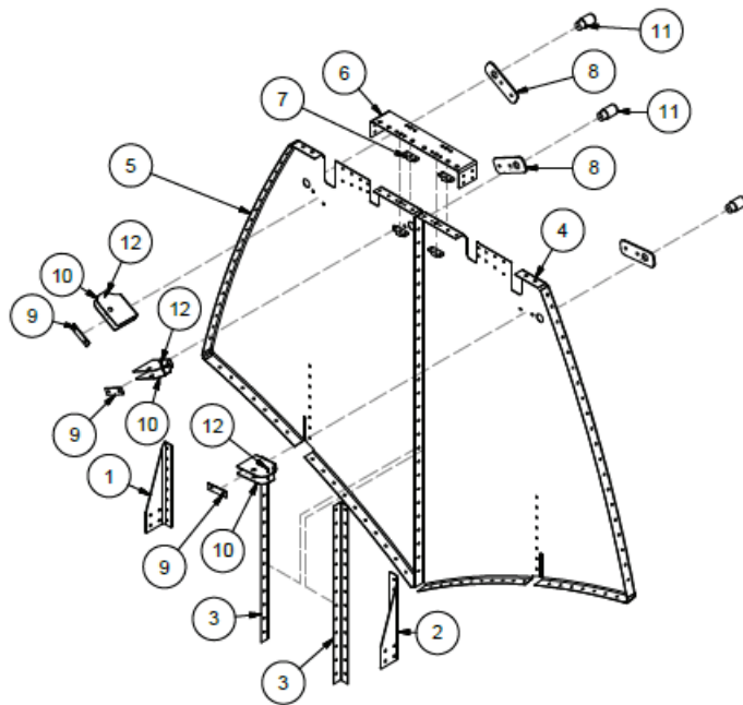
AFT SIDE
