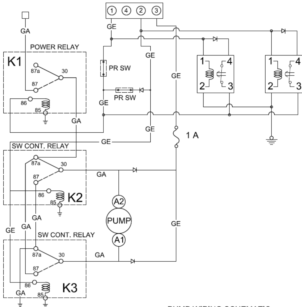
PUMP WIRING SCHEMATIC (RELAYS SHOWN IN RELAXED CONDITION)
