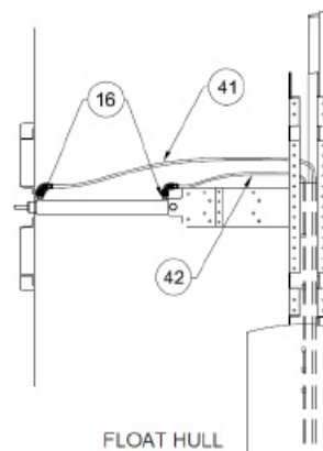
FLOAT HULL
