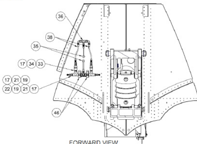
FORWARD VIEW
