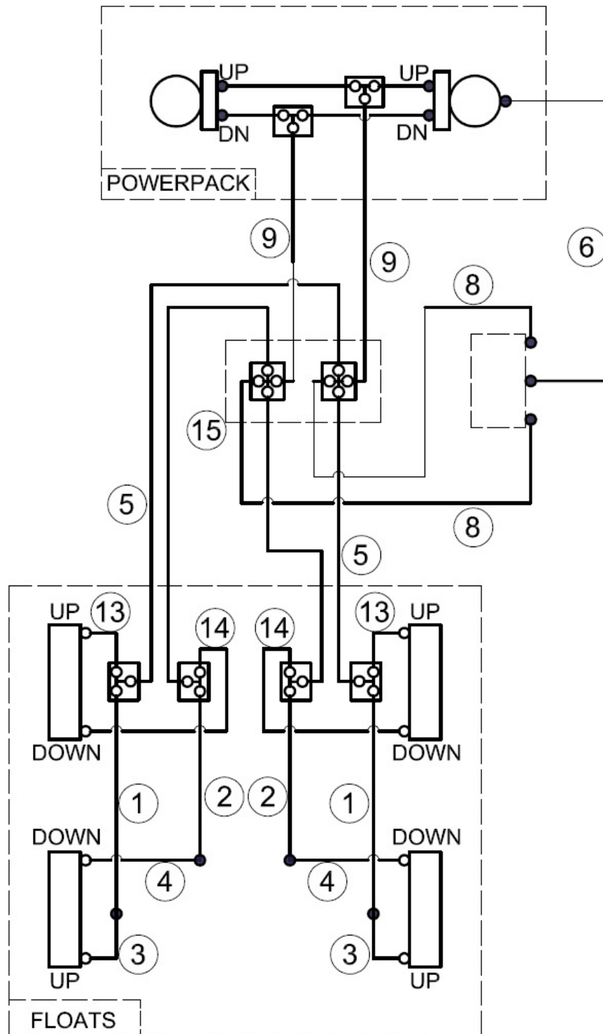
208 HYDRAULIC SCHEMATIC, BI-DIRECTIONAL
