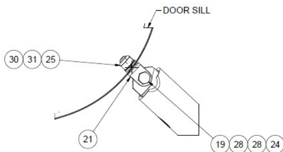
SECTION C-C CARGO DOOR AFT STEP STRUT EYEBOLT INSTALLATION
