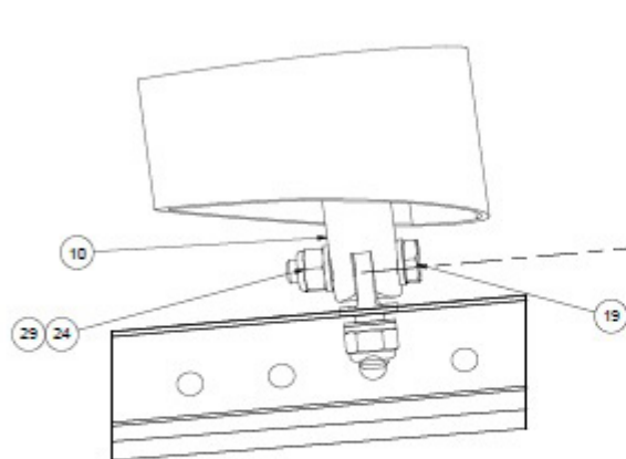
STRUT TO FLOAT DECK INSTALLATION (4 PLACES)
