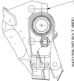
SECTION B-B PYLONS, COMPRESSION TUBES AFT FLY WIRES, & SPREADER BAR
