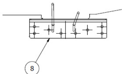
SECTION W INSTALL DOUBLER AND NOTCH OUT STIFFENER
