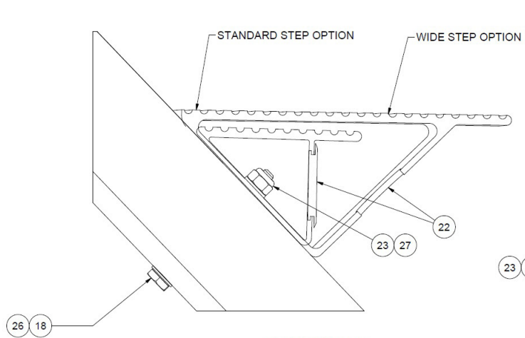
SECTION E-E FWD STRUT BOLTS (4 PLACES)
