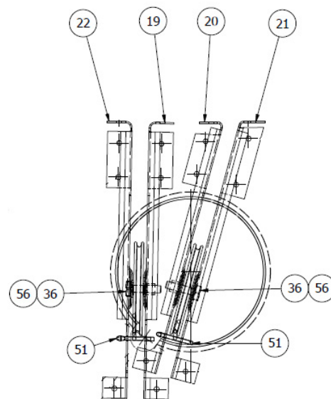
SECTION R INSTALL PULLEY BRACKETS, STA 344.00
