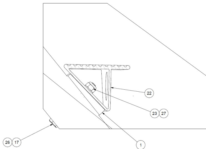
SECTION G-G PILOT/CO-PILOT AFT STEP STRUT (4 PLACES)
