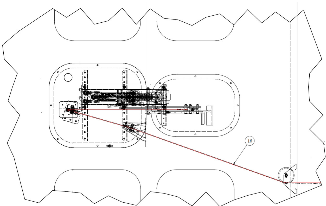
DETAIL A 1005706 AMPHIB RETRACT HANDLE
