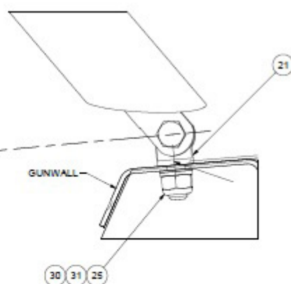
SECTION D-D FLOAT DECK EYEBOLT INSTALLATION PILOT-CO-PILOT/AFT CARGO STEP (3 PLACES)
