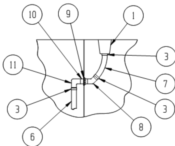
BULKHEAD #11 & #18
