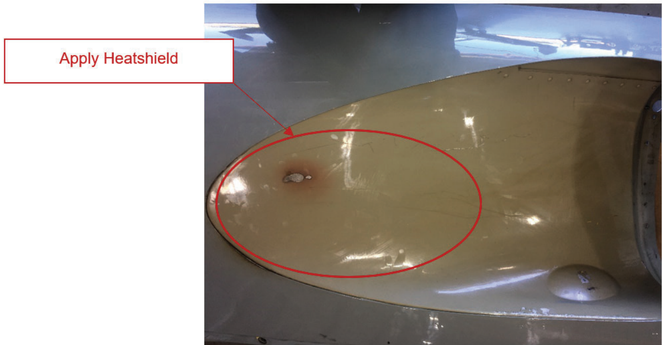
Figure 4 - Heatshield Area
