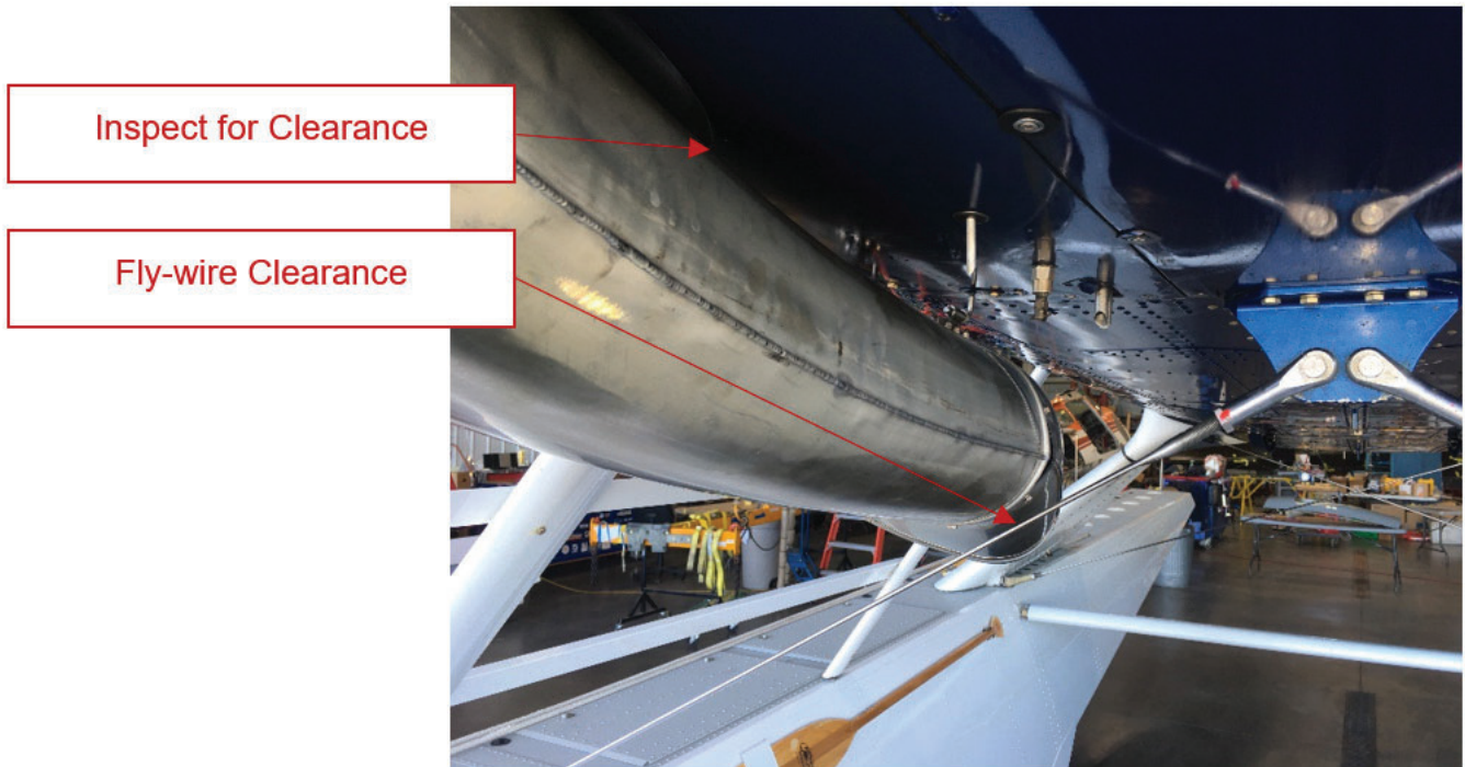
Figure 3 - Fly-wire Clearance
