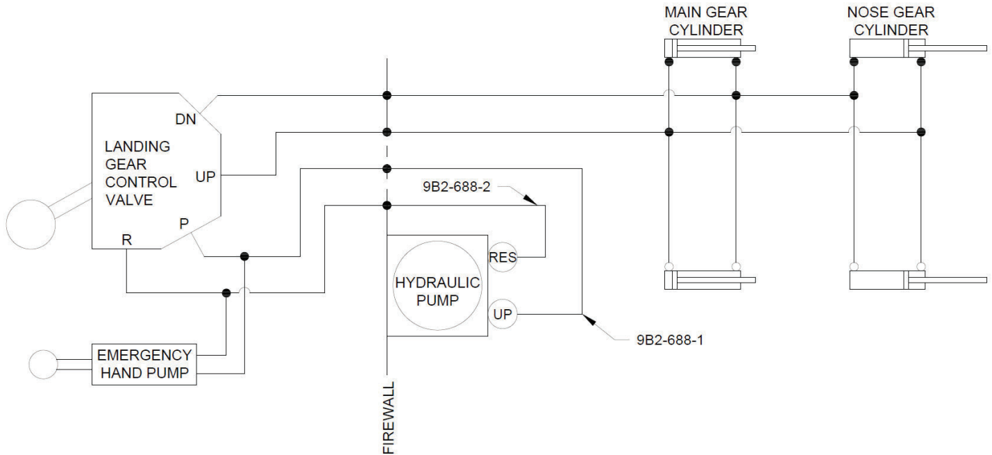
HYDRAULIC SCHEMATIC
