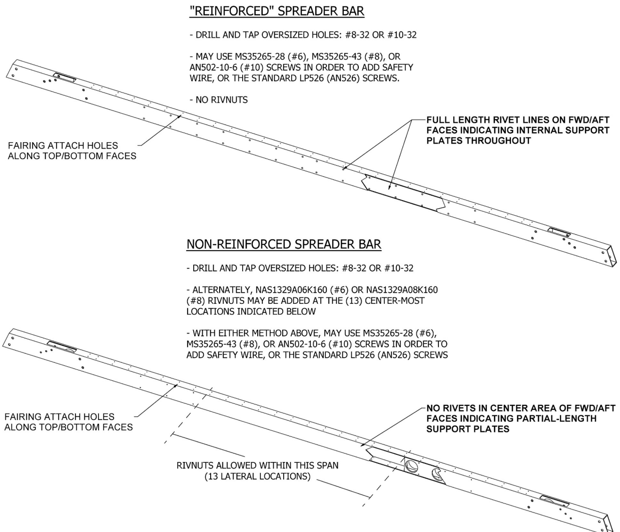
FIGURE 7.1: 8000 SPREADER BAR THREADED FAIRING HOLE REPAIR
