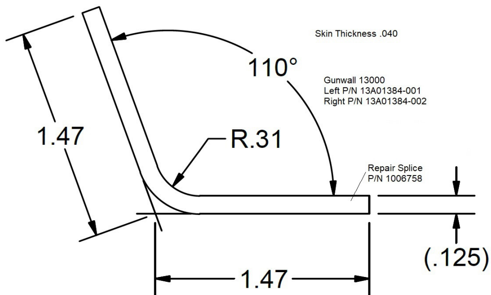
FIGURE 5.10-3: 13000 GUNWALL REPAIR
